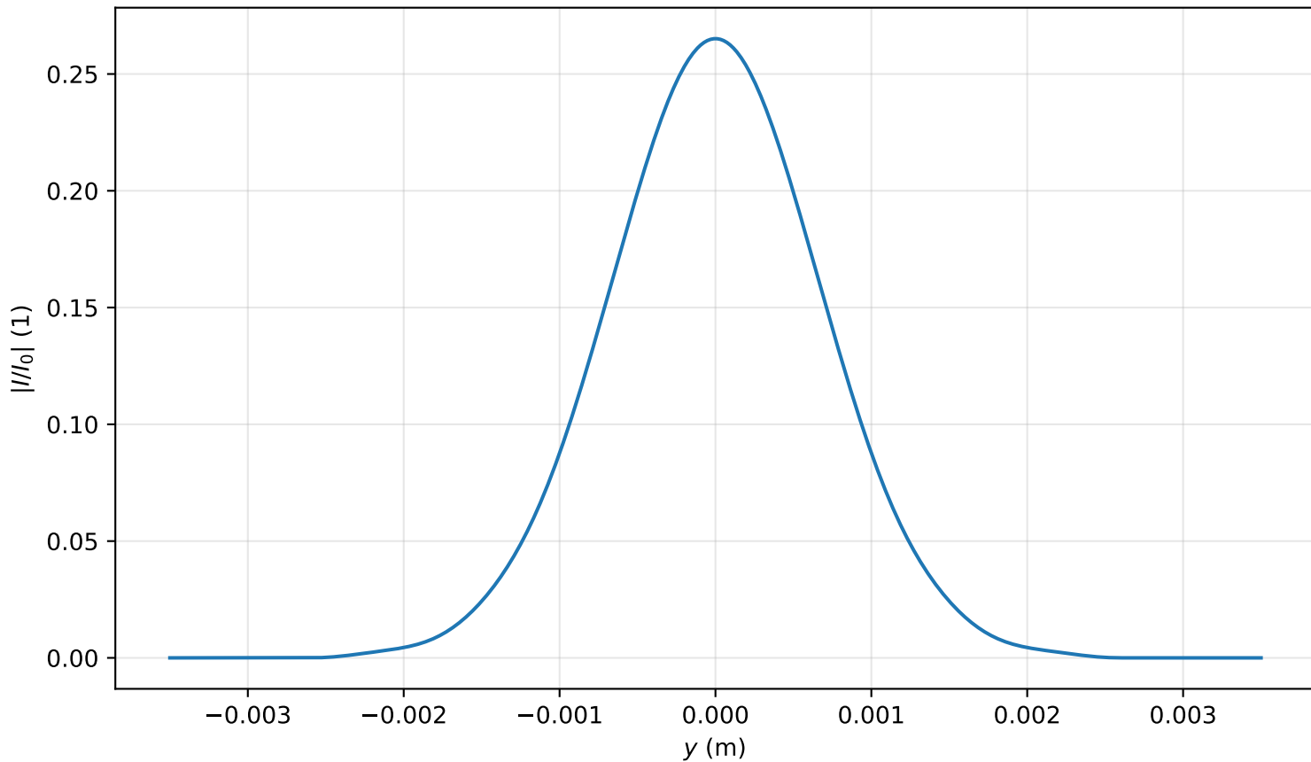
Intensity profile I(x=0, y, z=3.821)/I_0 , P_{in}=0.2P_{cr} , artificial time
